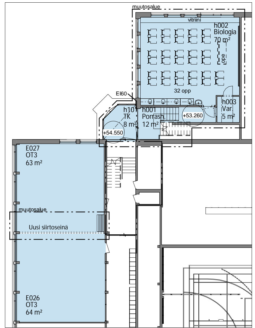
0. KRS 1/200_H-osa(FY-KE-BI) +53.260 1 : 200
