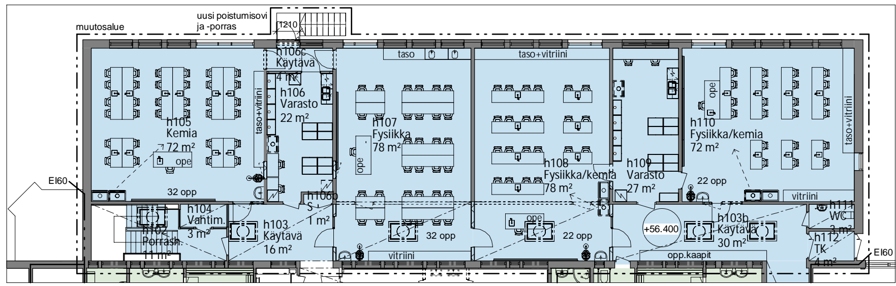
1. KRS 1/200_H-osa(FY-KE-BI) +56.400 1 : 200
